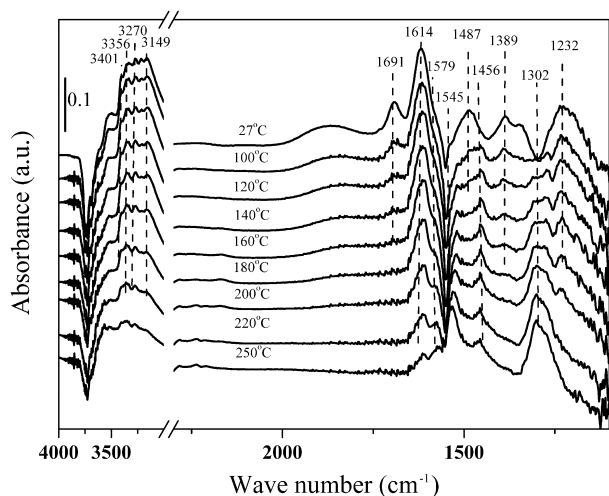
Fig. 6. FTIR spectra of the fresh 10 wt.% Ag/Al 2 O 3 catalyst treated with a flow of 500 ppm NH 3 + 10 vol.% O 2 /N 2 at various temperatures.
