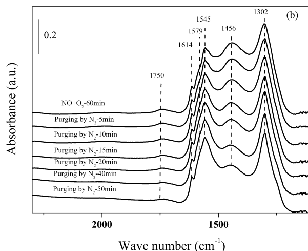
Fig. 10. FTIR spectra of the adsorbed species arising from \text{NO} + \text{O}_2 (500 ppm NO, \text{O}_2 10 vol.%) adsorption over the \text{H}_2 -pretreated 10 wt.% \text{Ag}/\text{Al}_2\text{O}_3 at 160^\circ\text{C} (a) and after successive purging with \text{N}_2 at 160^\circ\text{C} (b).
