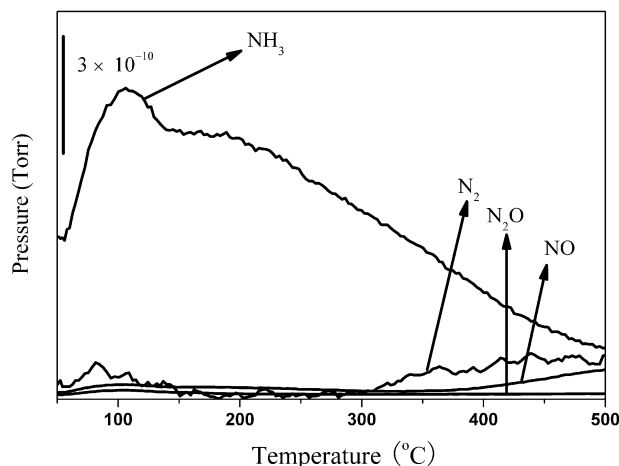
Fig. 3. \text{NH}_3 -TPO profiles over the fresh 10 wt.% \text{Ag}/\text{Al}_2\text{O}_3 catalyst, reaction conditions: \text{NH}_3 , 500 ppm; He as carrier; flow rate, 100 \text{cm}^3 \text{min}^{-1} ; catalyst weight, 0.1 g ( \text{W}/\text{F} = 0.06 \text{ g s cm}^{-1} ).
