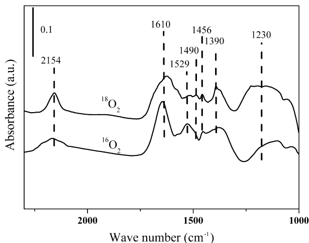
Fig. 9. FTIR spectra of the adsorbed \text{NH}_3 interacting with the ^{16}\text{O}_2 and ^{18}\text{O}_2 over \text{H}_2 -pretreated 10 wt.% \text{Ag}/\text{Al}_2\text{O}_3 at 100^\circ\text{C} (The sample was exposed to 20 Torr \text{NH}_3 for 30 min firstly, and then it was out gassed and exposed to 30 Torr \text{O}_2 ).
