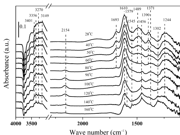
Fig. 7. FTIR spectra of the H 2 -pretreated 10 wt.% Ag/Al 2 O 3 catalyst treated with a flow of 500 ppm NH 3 + 10 vol.% O 2 /N 2 at various temperatures.
