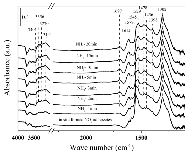
Fig. 11. FTIR spectra of the surface species arising from the interaction of \text{NH}_3 (500 ppm) with the in situ-formed \text{NO}_x on the \text{H}_2 -pretreated 10 wt.% \text{Ag}/\text{Al}_2\text{O}_3 at 160^\circ\text{C} .
