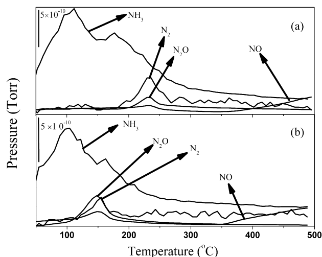
Fig. 1. NH 3 temperature-programmed oxidation (NH 3 -TPO) profiles over fresh (a) and H 2 -pretreated (b) 10 wt.% Ag/Al 2 O 3 catalysts. Reaction conditions: NH 3 , 500 ppm; O 2 , 10 vol.%; He as carrier; flow rate, 100 cm 3 min -1 ; catalyst weight, 0.1 g (W/F = 0.06 g s cm -1 ).
