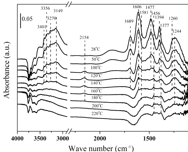
Fig. 5. FTIR spectra of the adsorbed species arising from contact of \text{NH}_3 (500 ppm) with the \text{H}_2 -pretreated 10 wt.% \text{Ag}/\text{Al}_2\text{O}_3 at room temperature and successive purging with \text{N}_2 at various temperatures.
