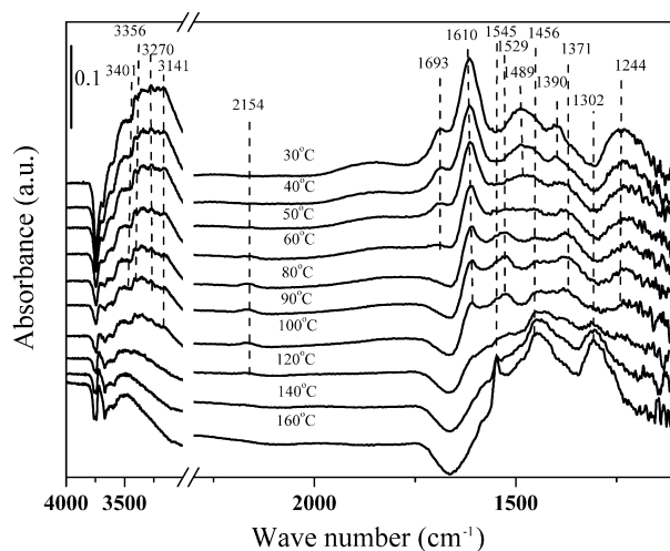
Fig. 8. FTIR spectra of the H 2 -pretreated 10 wt.% Ag/Al 2 O 3 taken after adsorption of NH 3 (500 ppm) at room temperature, followed by purging with N 2 for 30 min and successive heating in 10 vol.% O 2 /N 2 at various temperatures.
