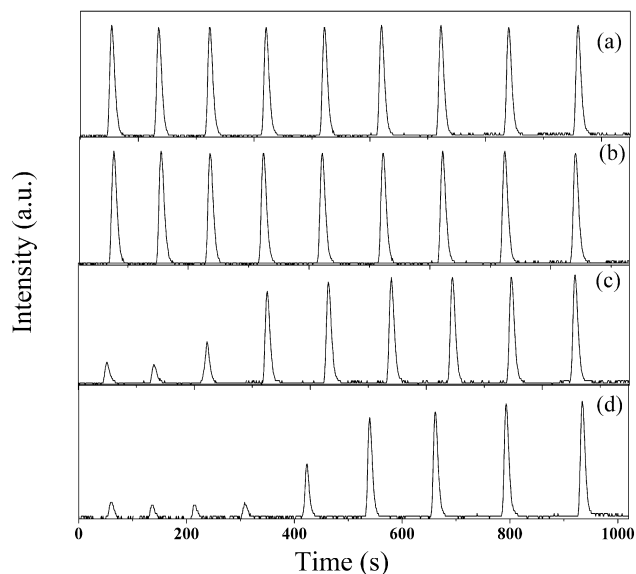
Fig. 2. \text{O}_2 uptakes on fresh 10 wt.% \text{Ag}/\text{Al}_2\text{O}_3 and on \text{H}_2 -pretreated 10 wt.% \text{Ag}/\text{Al}_2\text{O}_3 at various temperatures. Fresh 10 wt.% \text{Ag}/\text{Al}_2\text{O}_3 : 100 °C (a), 160 °C (b); \text{H}_2 -pretreated 10 wt.% \text{Ag}/\text{Al}_2\text{O}_3 : 100 °C (c); 160 °C (d). Reaction conditions: \text{O}_2 , 4.46 \mu\text{mol}/\text{pulse} ; He as carrier; flow rate, 40 \text{cm}^3 \text{min}^{-1} ; catalyst weight, 0.3 g.
