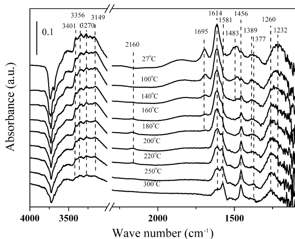
Fig. 4. FTIR spectra of the adsorbed species arising from contact of \text{NH}_3 (500 ppm) with the fresh 10 wt.% \text{Ag}/\text{Al}_2\text{O}_3 at room temperature and successive purging with \text{N}_2 at various temperatures.
